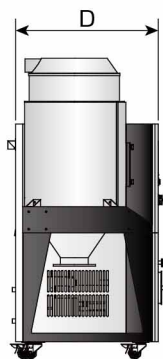
SDD-300U/200H~1200U/700H
